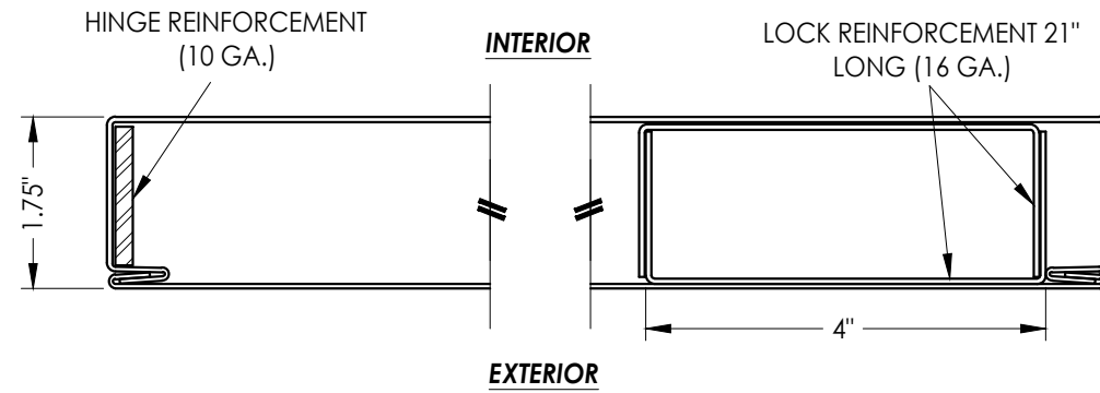
1 HORIZONTAL CROSS SECTION 3
